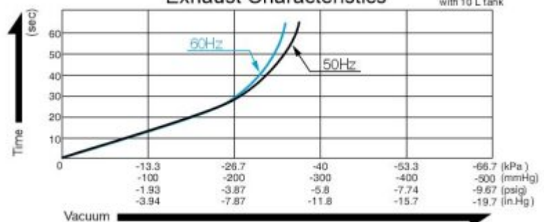
Exhaust Characteristics
